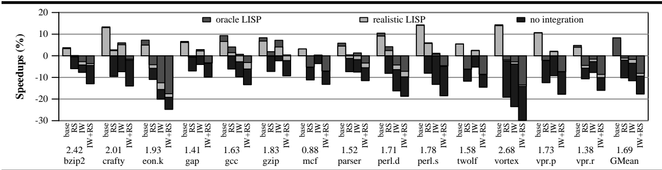
FIGURE 7. Impact of integration on reduced-complexity execution engines
