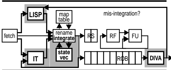
FIGURE 1. Register integration implementation
