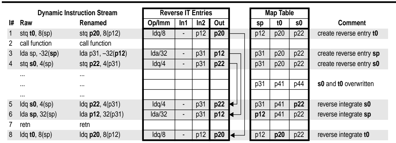
FIGURE 3. Speculative memory bypassing via reverse integration
