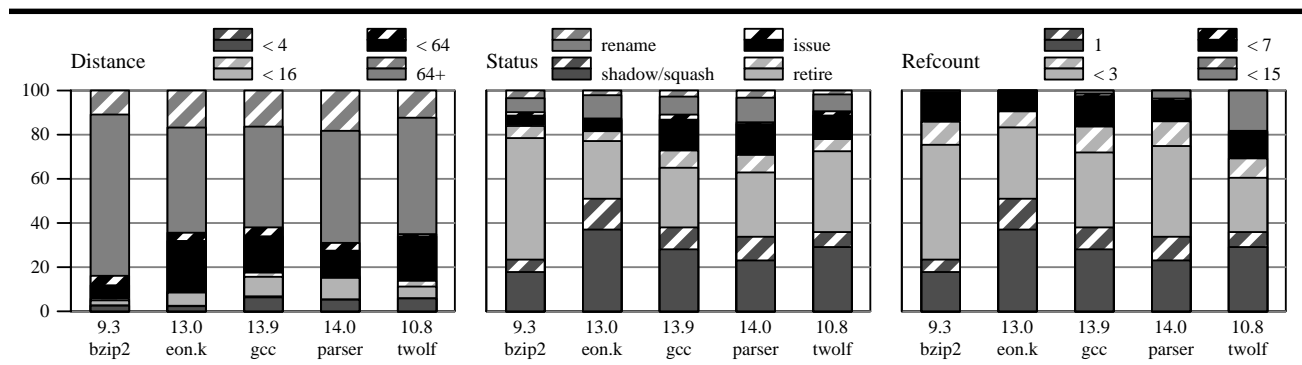
FIGURE 5. Breakdowns of integration retirement stream
