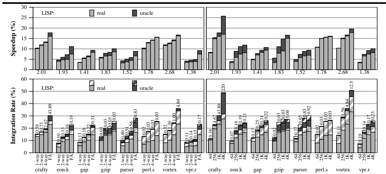
FIGURE 6. Impact of IT associativity and size
