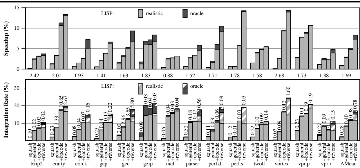
FIGURE 4. Impact of general reuse, opcode indexing, and speculative memory bypassing
